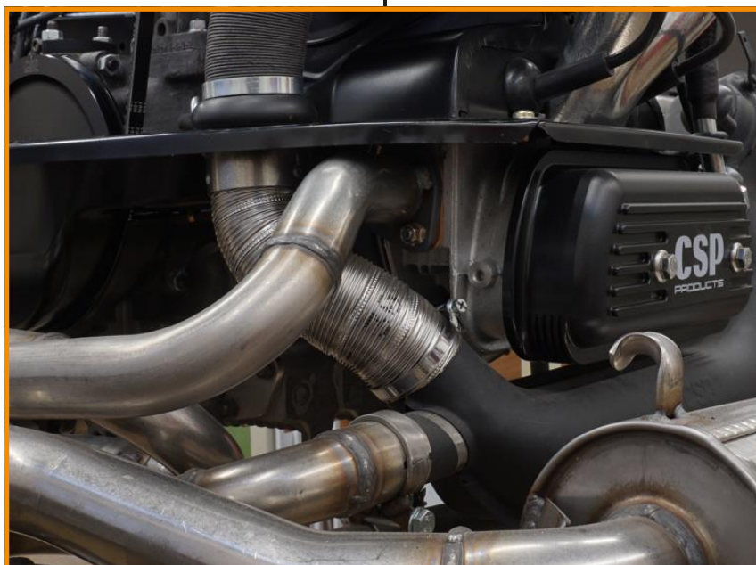
Fig. 6 Anschluss der Heizschlauchanschlüsse Mounting of heater hose fittings
